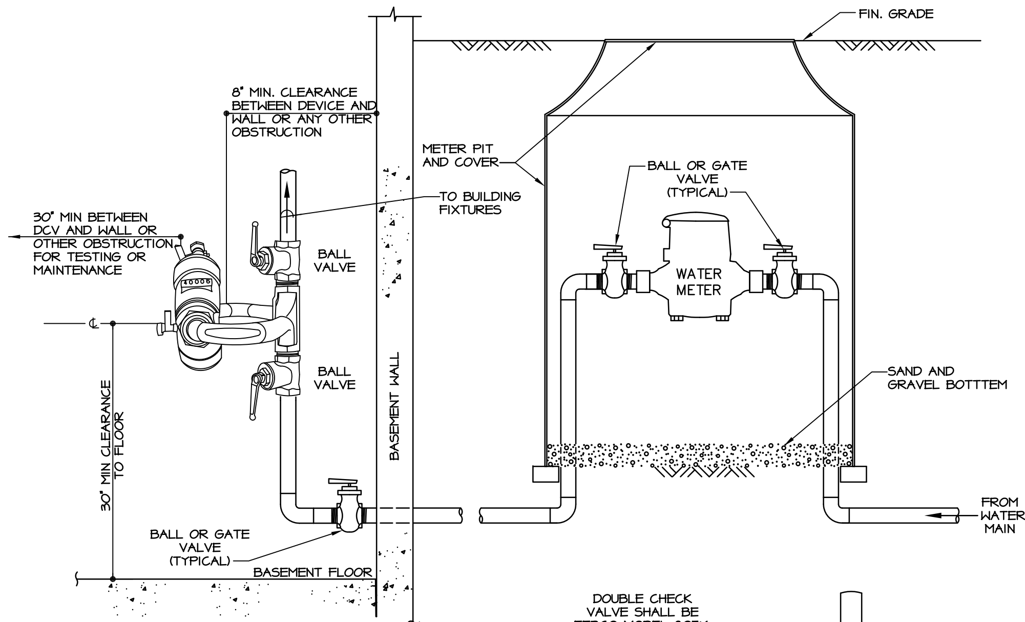
ELEVATION NO SCALE
