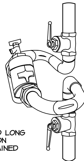
ANGLE VIEW SHOWING SEPARATION OF ELBOW NO SCALE
