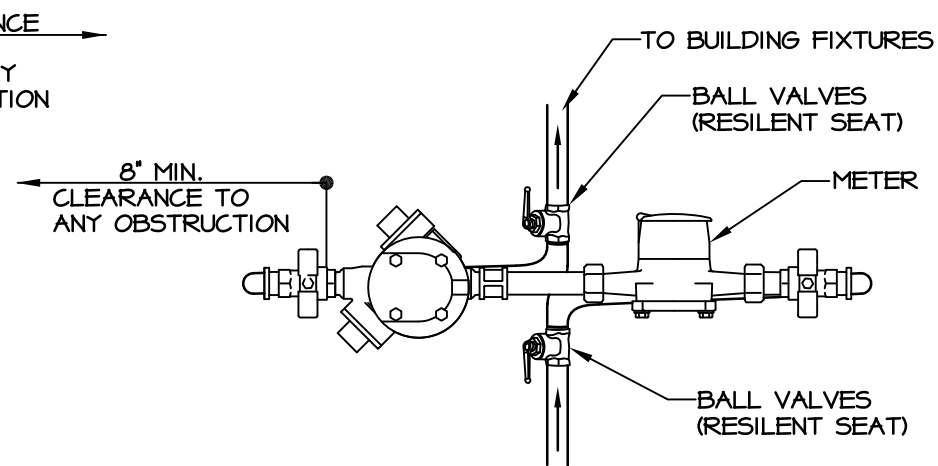
FRONT VIEW NO SCALE
