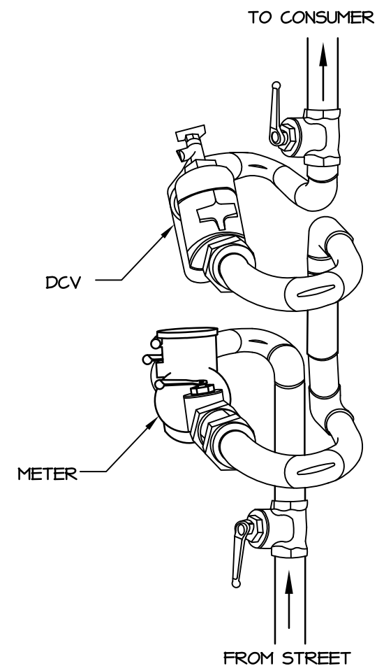
ANGLE VIEW SHOWING SEPARATION OF ELBOW NO SCALE
